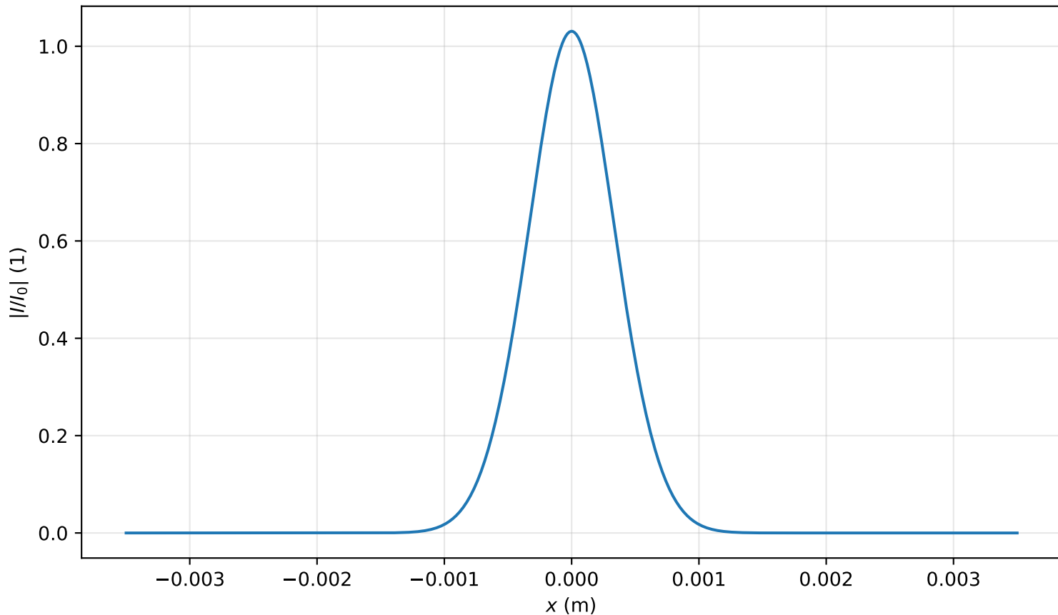
Intensity profile I(x, y = 0, z = 0.239m)/I_0 , P_{in}=0.8P_{cr} , artificial time
